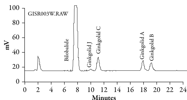
Figure 1. High-performance liquid chromatography (HPLC) fingerprint of ginkgolides and bilobalide from the ginkgo fresh plant extract.
