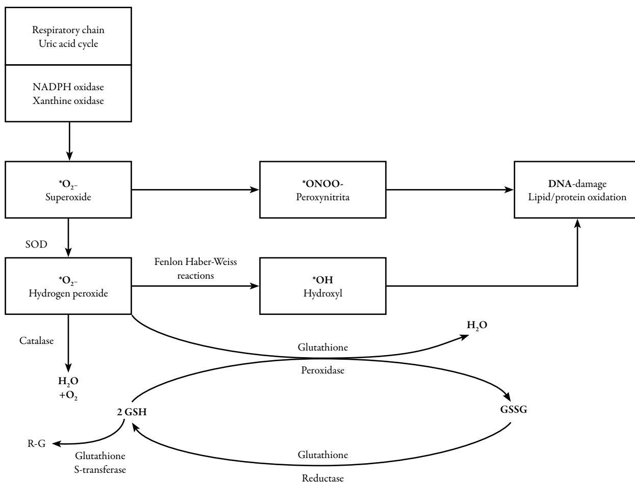
Figure 7. Scheme of the production of free oxygen radicals and their elimination and detoxification by superoxide dismutase (SOD), catalase, and glutathione peroxidase. Increased amounts of reduced glutathione (two glutathione [GSH]) are mostly caused by SOD upregulation. GSSG=glutathione disulphide; NADPH=nicotinamide adenine dinucleotide phosphate; OH=hydroxide; ONOO=peroxynitrite. Diagram adapted from Siegel et al. 19 with friendly permission of Springer Verlag, Vienna, which also owns the copyright for this figure.
